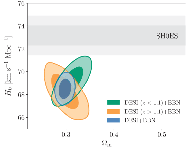
FIG. 9. Comparison of our H_0 constraints with respect to SH 0 ES, assuming a \Lambda CDM model (Sec. VI). We show the combination DESI + BBN for our low redshift and high redshift samples. For z > 1.1 , only the ELG2, QSO, and Ly \alpha tracers are included, while DESI( z < 1.1 ) includes BGS, LRGs and the LRG3+ELG1 tracer combinations. Both subsets are individually in > 3\sigma tension with SH 0 ES measurements.
