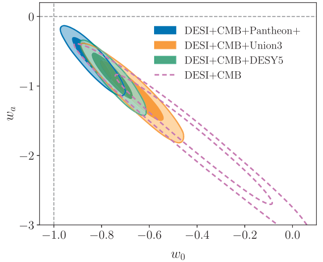
FIG. 11. Results for the posterior distributions of w_0 and w_a , from fits of the w_0w_a CDM model to DESJ in combination with CMB and three SNe datasets as labeled. We also show the contour for DESJ combined with CMB alone. The contours enclose 68% and 95% of the posterior probability. The gray dashed lines indicate w_0 = -1 and w_a = 0 ; the \Lambda CDM limit ( w_0 = -1 , w_a = 0 ) lies at their intersection. The significance of rejection of \Lambda CDM is 2.8\sigma , 3.8\sigma and 4.2\sigma for combinations with the Pantheon+, Union3 and DESY5 SNe samples, respectively, and 3.1\sigma for DESJ + CMB without any SNe.
