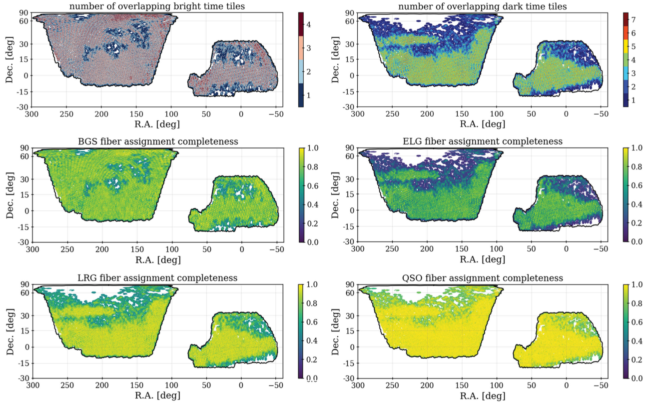
FIG. 2. Top two panels: the number of overlapping tiles in DR2 for bright and dark time. Lower four panels: the assignment completeness of the four DESI samples, within unique tile groupings. One can observe that the patterns in the completeness correspond to the number of overlapping tiles. The black outline shows the edges of the area within which DESI dark or bright tiles have been defined, as of 9 April 2024. The completeness maps can be compared to the values in Table II.
