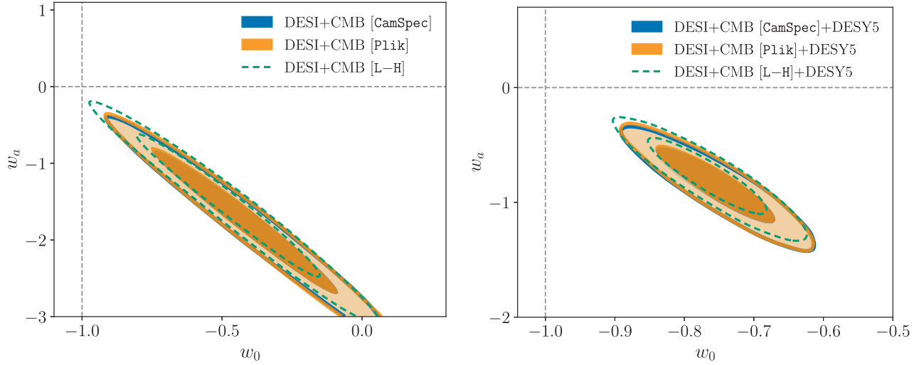
FIG. 18. Effect of changing the CMB likelihood between our default CamSpec, Planck, and L-H (see Sec. IV B for details), on results in the w_0 - w_a plane. Left: posteriors in the DESI + CMB case. Right: the case when also combining with DESY5 SNE information. The L-H likelihood shows a small shift compared to the other two likelihoods, but this difference is suppressed when also including SNE data.
